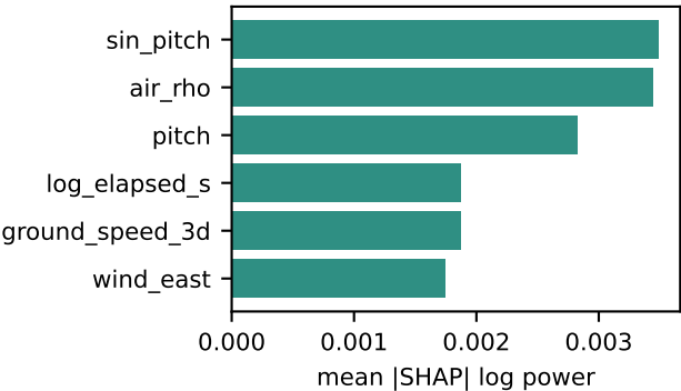
GradientExplainer SHAP audit (C7 limited)
