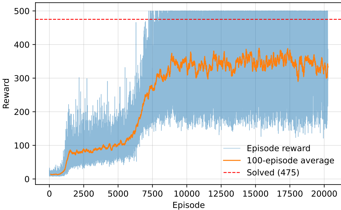
CartPole-v1 A2C Training Performance (Online)
