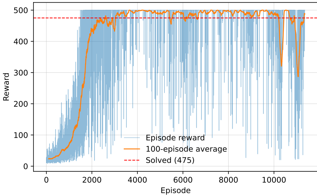
CartPole-v1 A2C Training Performance
