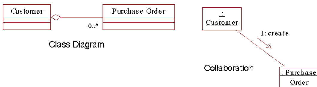
Figure 64 - Class Diagram and Collaboration for "Create Purchase Order" So, we have now coupled Customer and Purchase Order together. That is fine, because they are coupled together in real life too.
