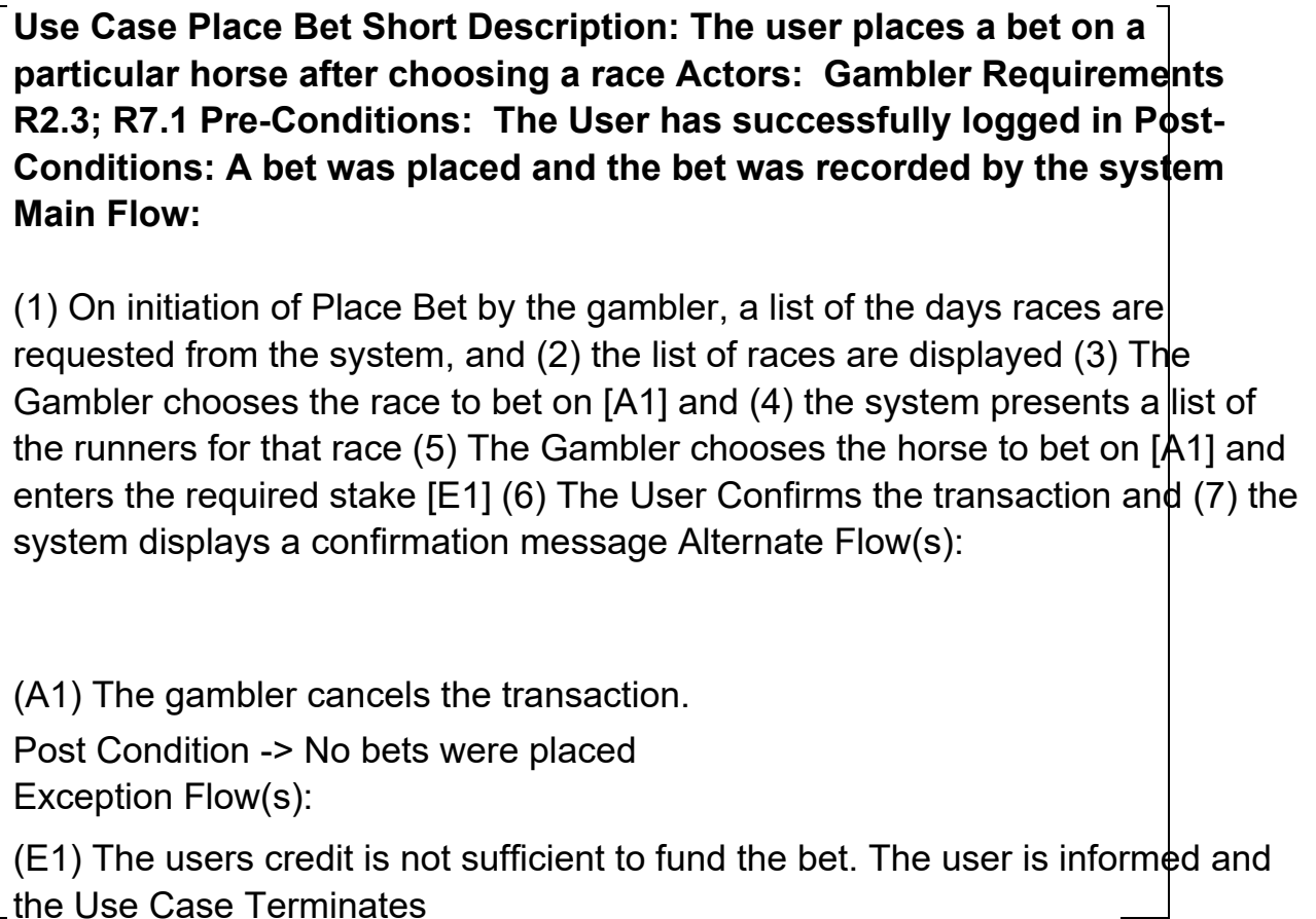
Figure 43 - Full Use Case Description
