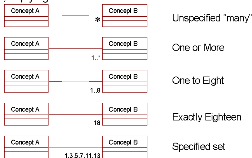
Figure 38 - Example Cardinalities
