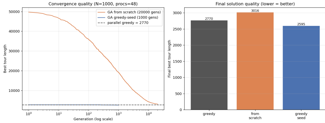
Figure 6: Quality experiment: convergence curves and final best tour length.
