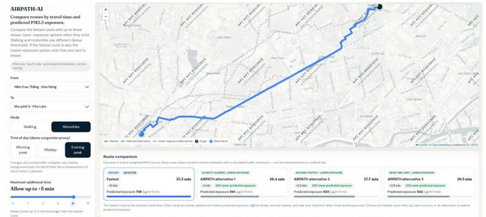
Fig. 2. AIRPATH-AI web prototype (motorbike, evening-peak demo window) for Hèm Cao Thăng · Hòa Hưng to Khu phố 11 · Phú Lâm, with the three-session time-of-day control visible in the sidebar.
