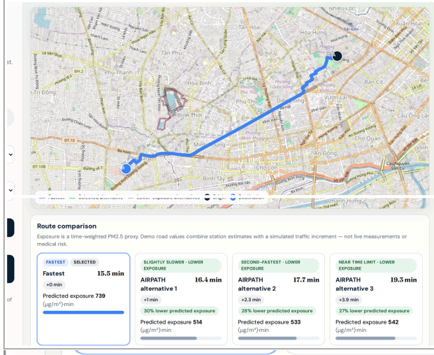
Fig. 2. AIRPATH-AI web prototype (motorbike, evening-peak demo window, +5 min): Hẻm Cao Thắng · Hòa Hưng to Khu phố 11 · Phú Lâm. High-resolution interface screenshot; the three-session control is a demo congestion proxy only (not Gap 1 or Gap 2).
