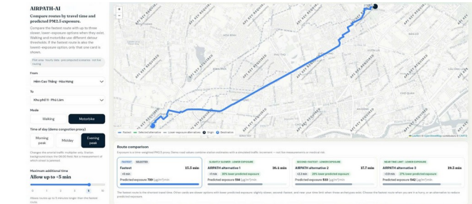
Fig. 2. AIRPATH-AI web prototype screenshot (motorbike, evening-peak demo window) for Hẻm Cao Thắng · Hòa Hưng to Khu phố 11 · Phú Lâm. The three-session control is a demo congestion proxy only; it is not Gap 1 or Gap 2.
