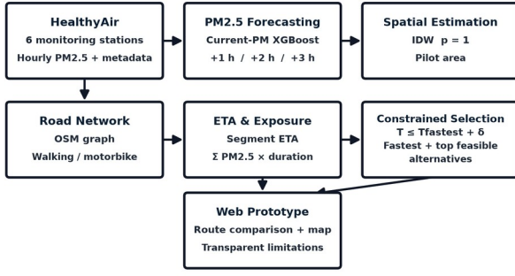
Fig. 1. AIRPATH-AI frozen research pipeline: station observations → forecasting → spatial estimation → road network/ETA → exposure → constrained route selection → web prototype.
