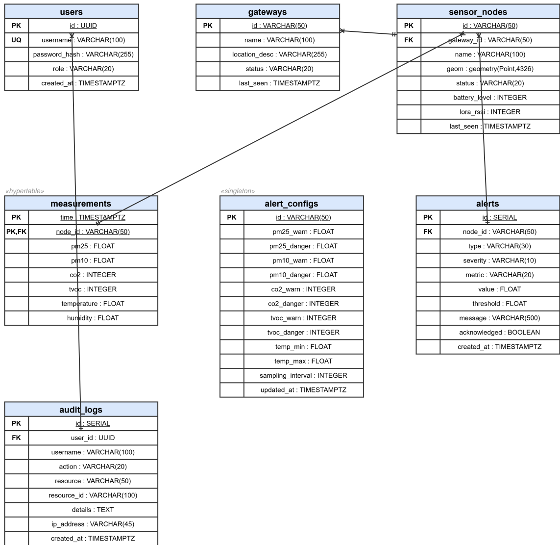
Hình 0.9: Entity-Relationship Diagram
