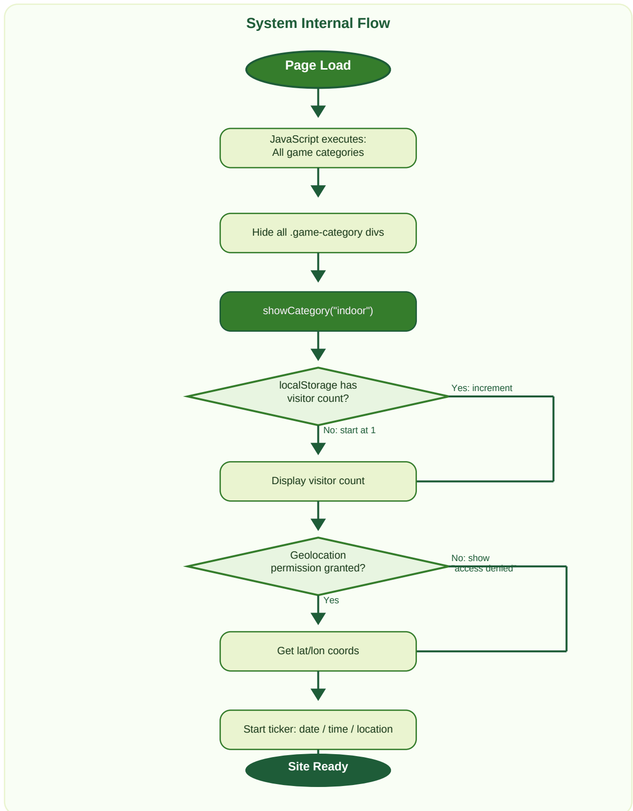
Figure 3: System Internal Flow on Page Load
