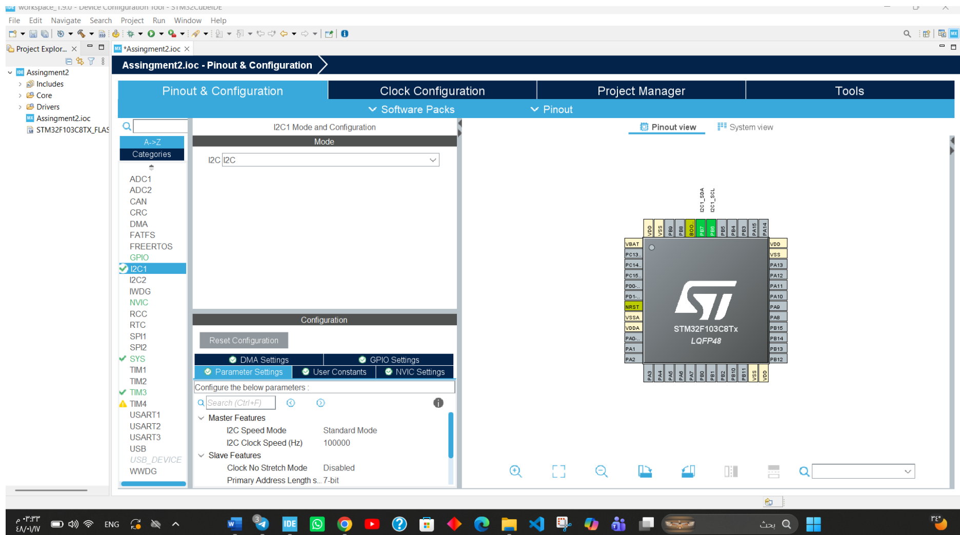
Figure 2 I2C1 Configuration for TC74 Sensor
