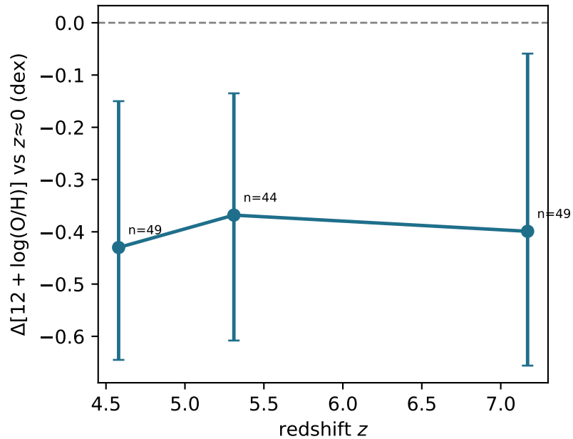
Metallicity deficit ( T_e scale)
