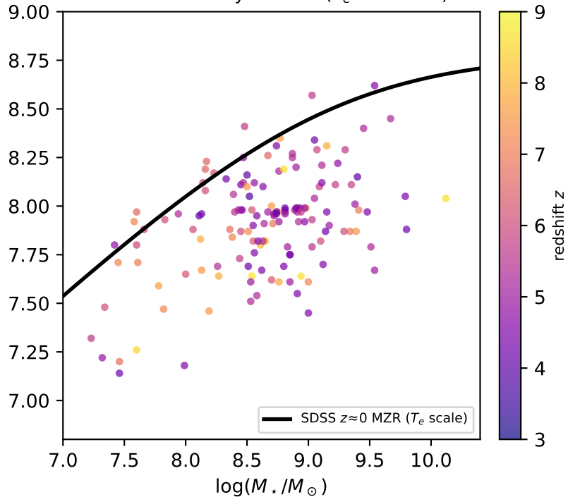
Mass--metallicity relation ( T_e -anchored)
