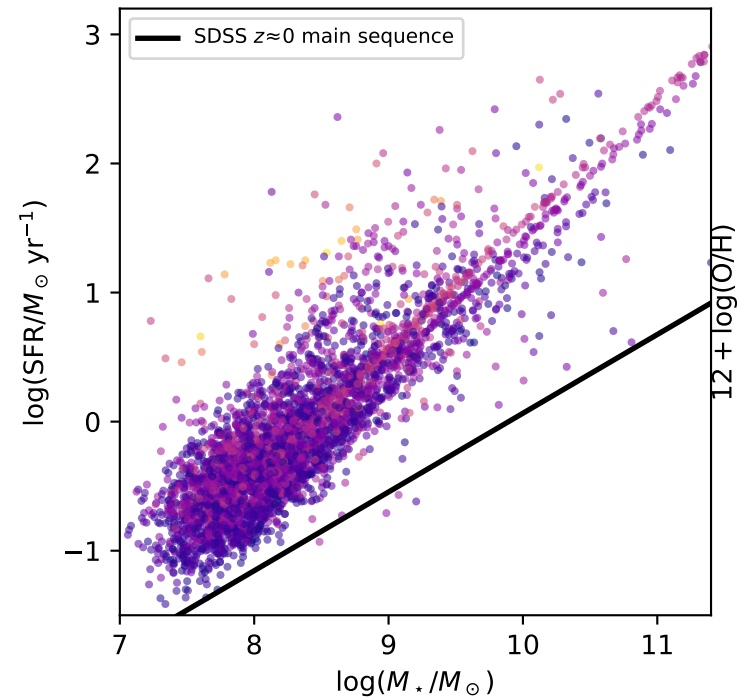
Star-forming main sequence
