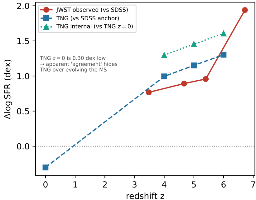
Main-sequence elevation
