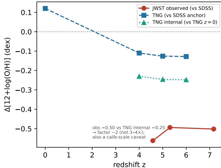
Metallicity offset
