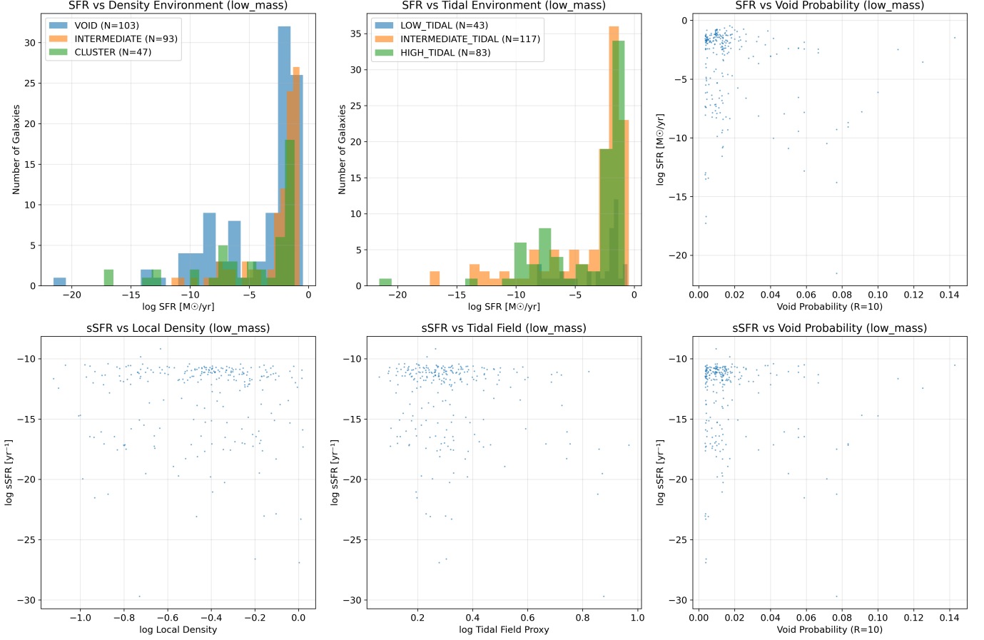
Figure 2. Environmental effects on star formation for low-mass galaxies ( \log M_* \lesssim 10.0 M_\odot ). Top row: SFR distributions across density environments (left), tidal environments (center), and SFR versus void probability (right). Bottom row: sSFR correlations with local density (left), tidal field proxy (center), and void probability (right). Environmental effects are moderate in this mass range.
