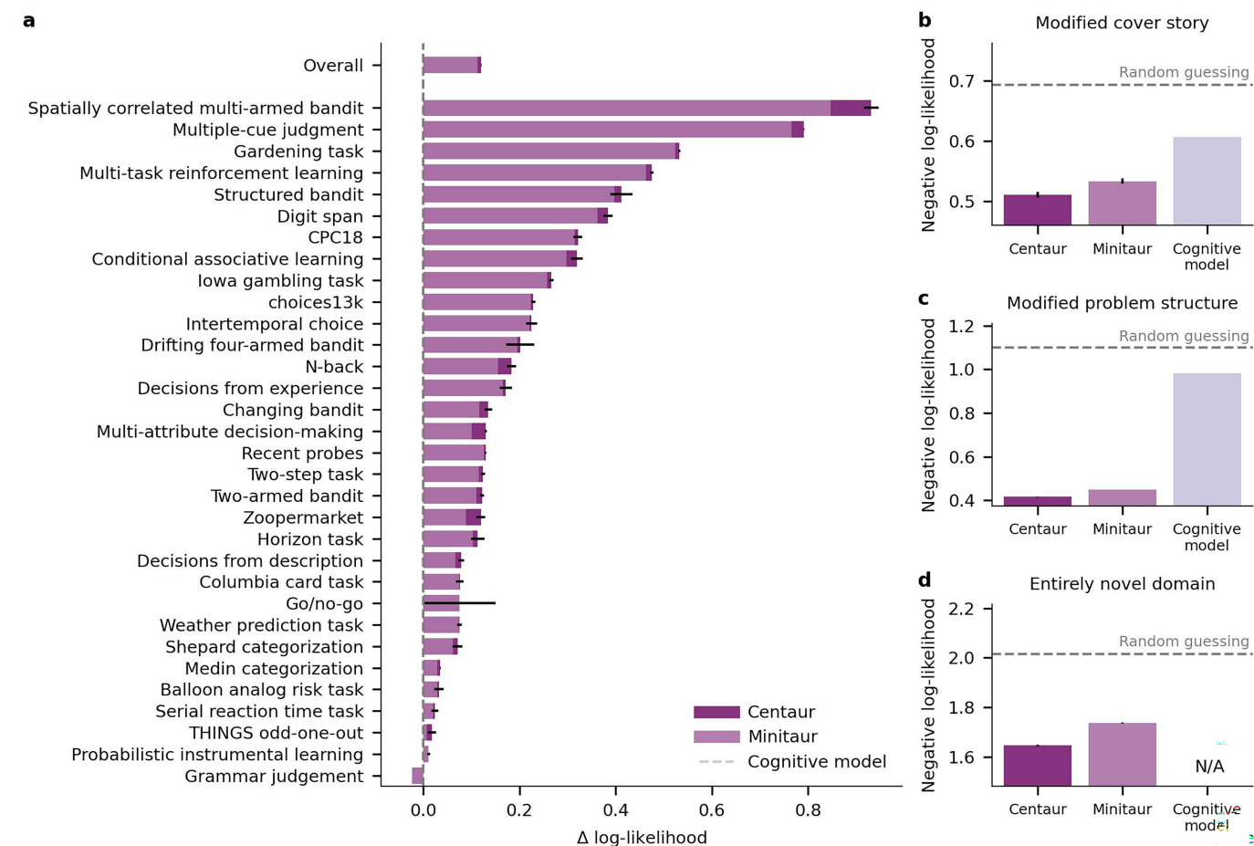
Extended Data Fig. 7 | Log-likelihood comparison between Centaur and Minitaur on the analyses from the main text. a, Negative log-likelihoods relative to the domain-specific cognitive models on held-out participants from Psych-101. Error bars correspond to the standard error of the mean, taken over
