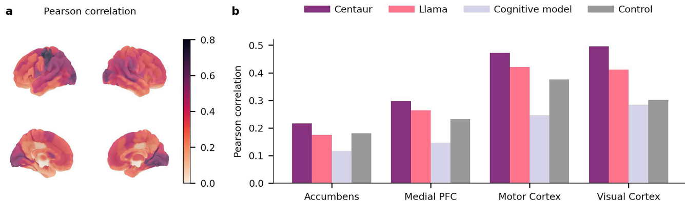
Extended Data Fig. 6 | Finegrained neural alignment results in the two-step task. a , Pearson correlation coefficients between the predicted activity from Centaur's representations and the BOLD data shown on a surface brain (image created with Nilearn 66 ). Centaur achieves the most accurate predictions in the left motor cortex. As participants performed the task with their right hand in the scanner, this effect may be explained by Centaur's strong performance in predicting choices. b , Predictive performance of Centaur's representations against alternatives for ROIs that have been identified as behaviorally relevant in previous work. Cortical scores are averaged over the
