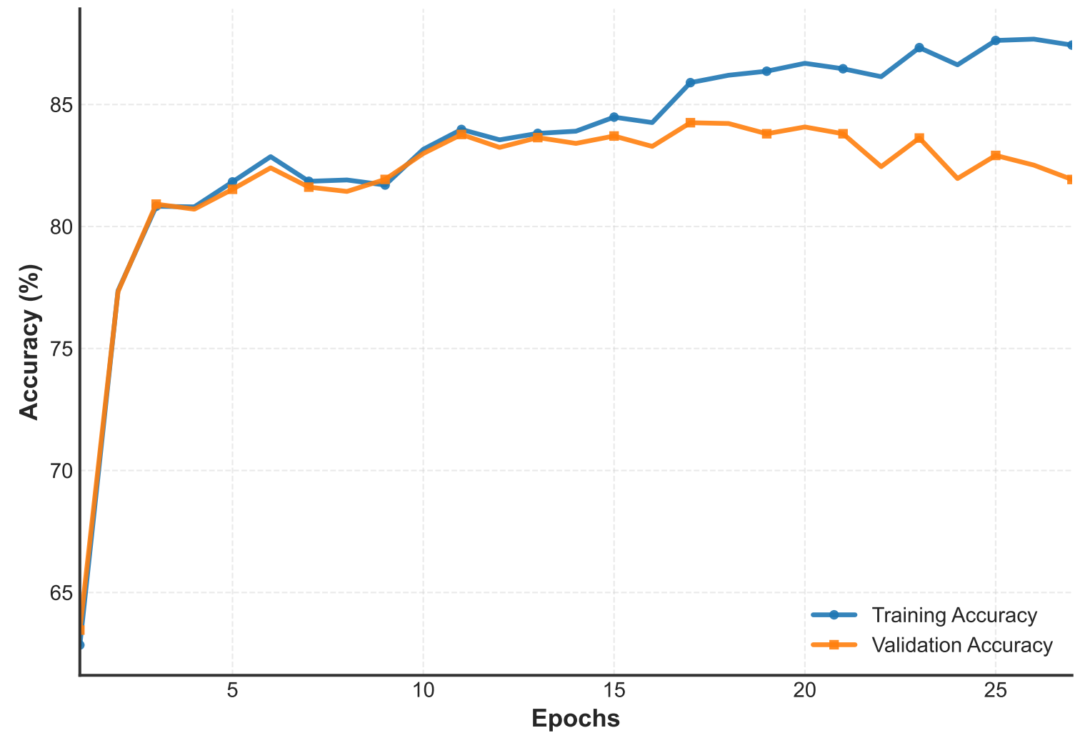
Training and Validation Accuracy (%)
