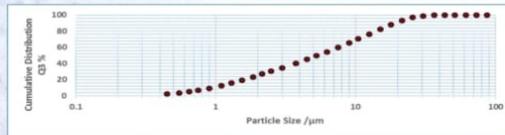
Particle Size Distribution (Sympatec HELOS/BF)
