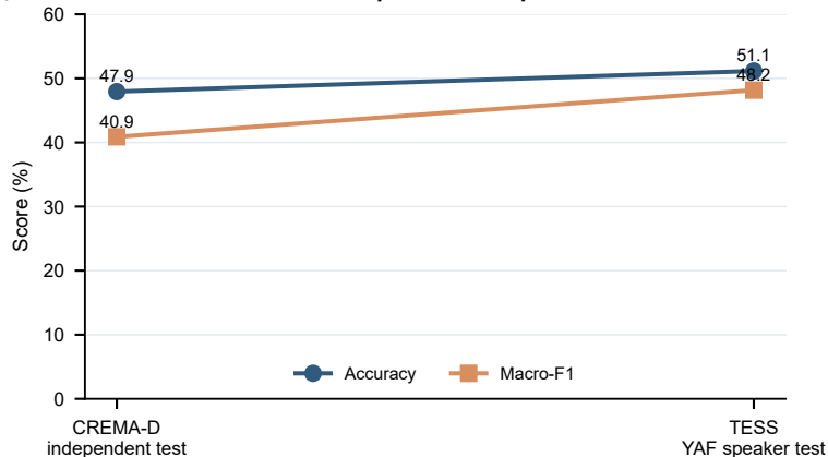
d Cross-corpus test comparison
