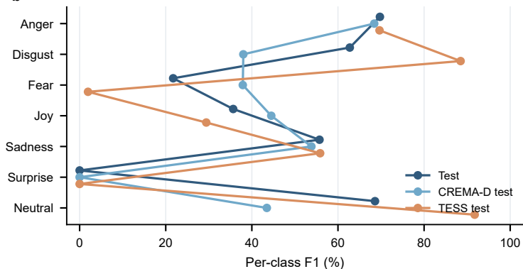
d Cross-corpus test comparison
