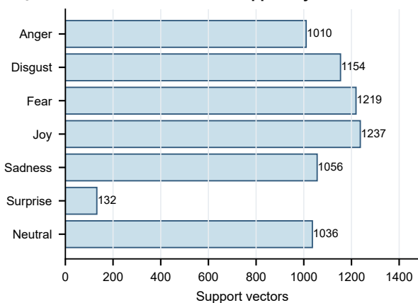
c SVM decision support by class
