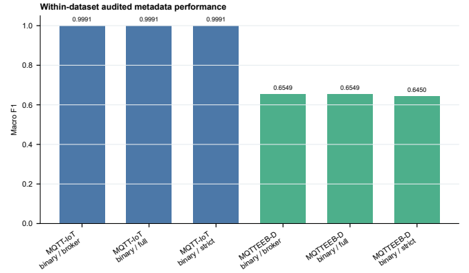
Fig. 4: Within-dataset Macro F1 for packet-level MQTTEEB-D and MQTT-IoT biflow audited views. MQTTEEB-D flow-window results are reported separately.
