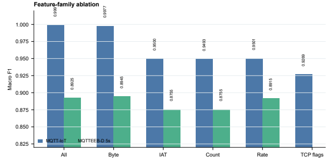
Fig. 7: Feature-family ablation for MQTT-IoT and MQTTEEB-D strict 5 s metadata.
