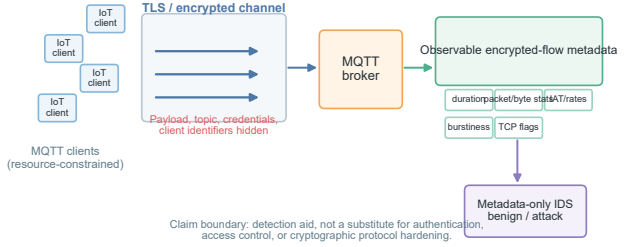
Fig. 1: Metadata-only IDS under encrypted MQTT monitoring. Payloads, topics, credentials, and client identities are hidden by encryption or privacy constraints, while encrypted-flow metadata remains observable.
