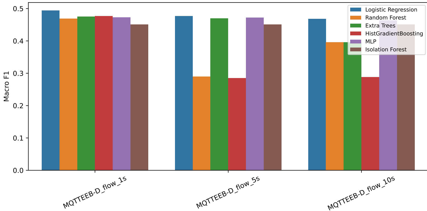
External validation: MQTTEEB-D to IoT-23
