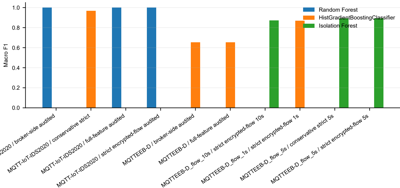
Crypto-observability ablation
