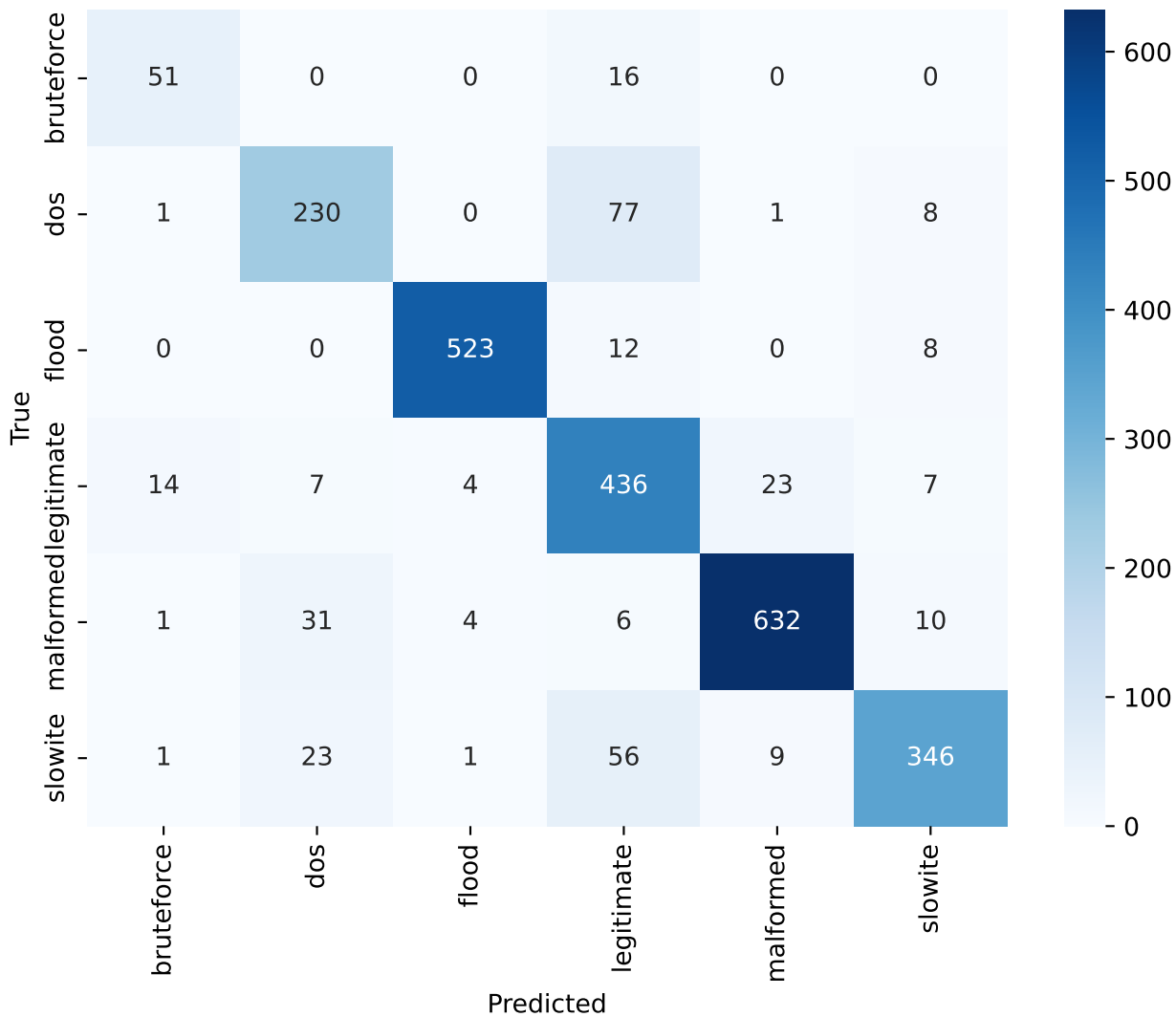
MQTTEEB-D best multiclass confusion matrix
