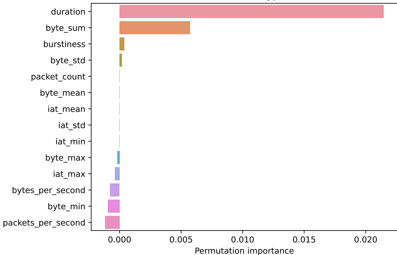
MQTTEEB-D strict encrypted-flow 5s
