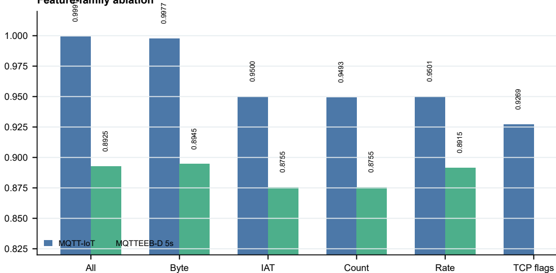
Feature-family ablation
