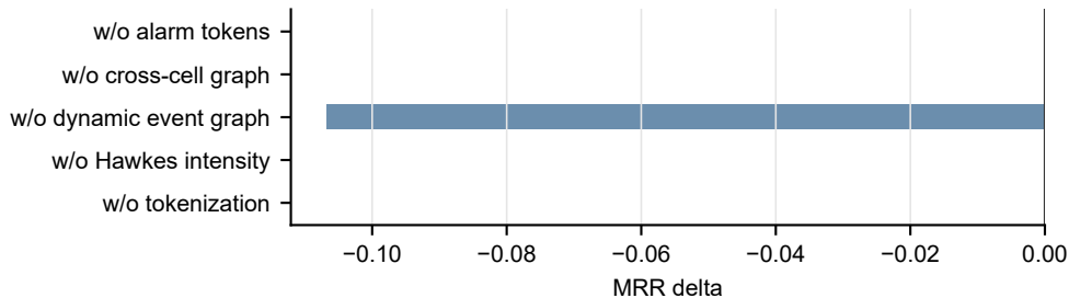
C. Weak ranking delta MRR
