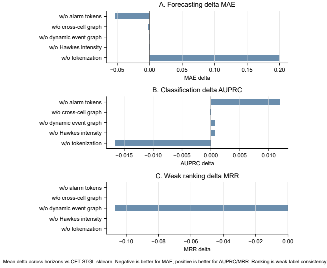
Fig. 3. Ablation deltas relative to CET-STGL-sklearn. Negative deltas are better for MAE, while positive deltas are better for AUPRC and MRR. Ranking deltas reflect weak-label/proxy consistency only.
