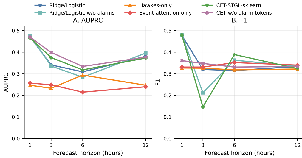
Figure 4: KPI degradation classification performance versus prediction horizon.
