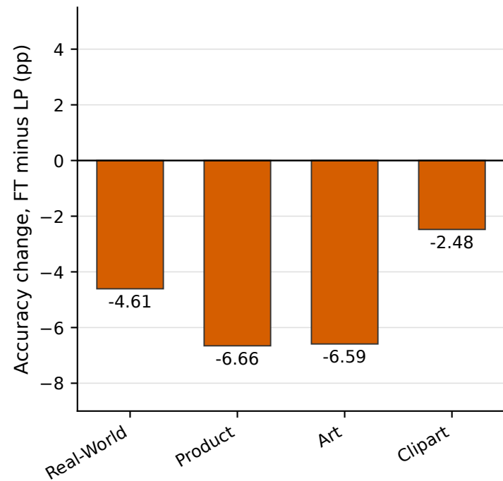
(a) ResNet18
