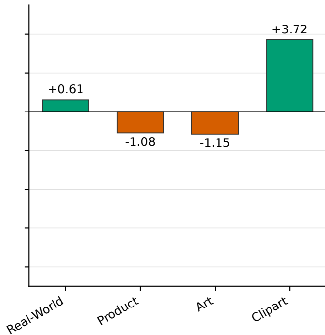
(b) ResNet50
