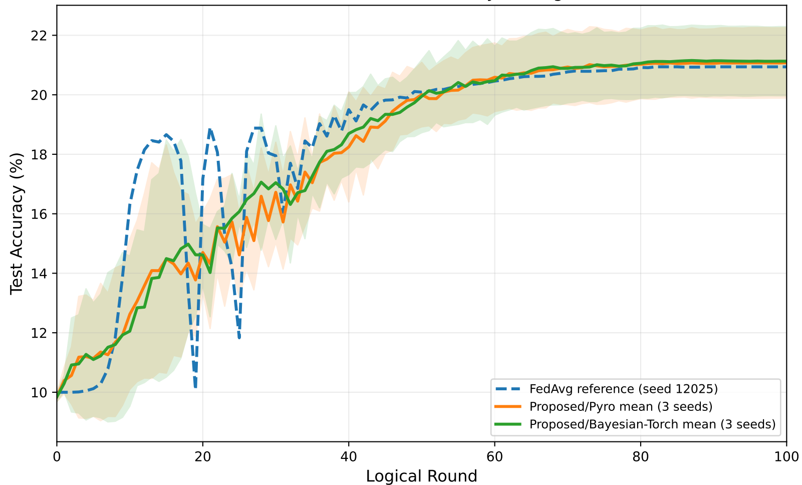
CIFAR-10 Dense Baseline: Accuracy vs. Logical Round
