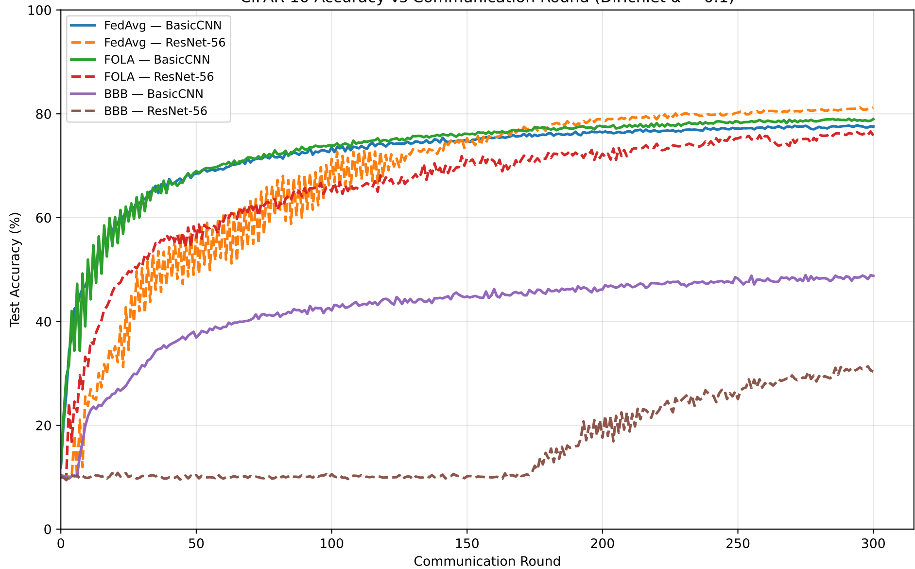
CIFAR-10 Accuracy vs Communication Round (Dirichlet \alpha = 0.1 )
