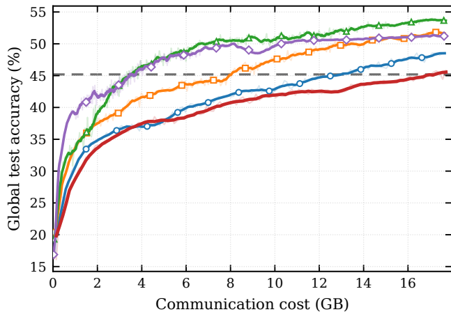
CIFAR-10
