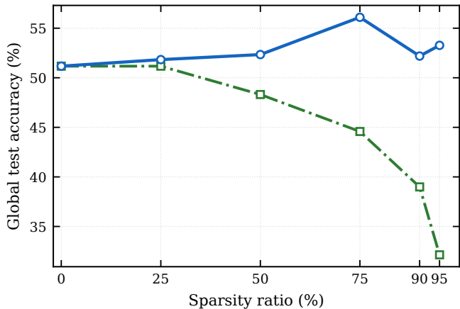
CIFAR-10
