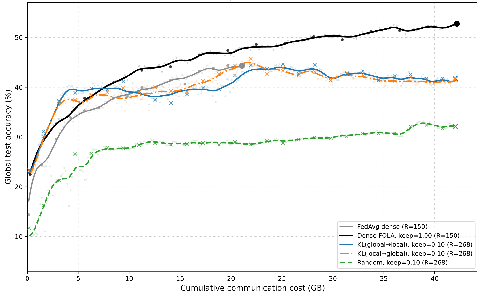
CIFAR-10 | \alpha=0.01 | local fraction=1.0 Keep ratio = 0.10
