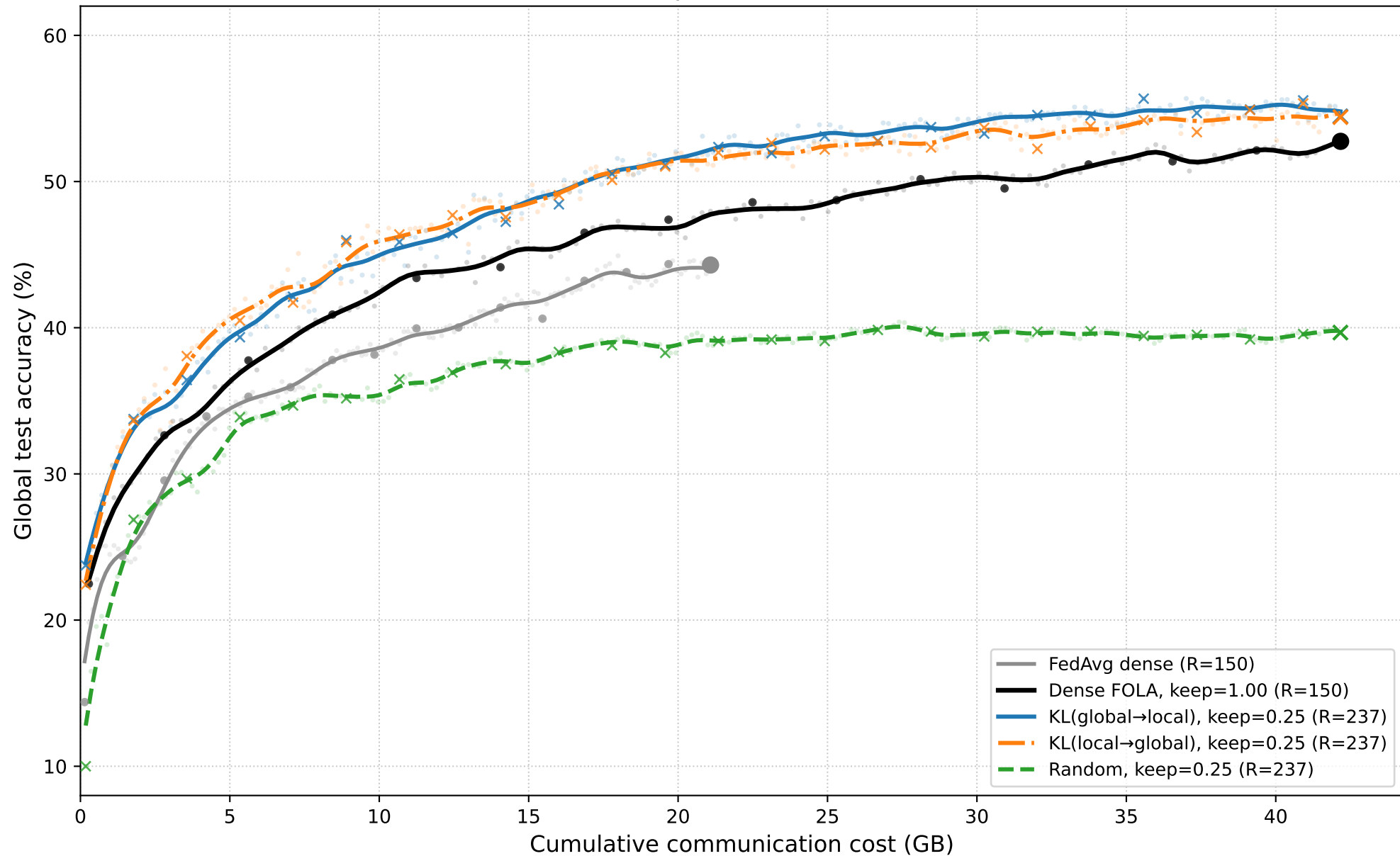
CIFAR-10 | \alpha=0.01 | local fraction=1.0 Keep ratio = 0.25
