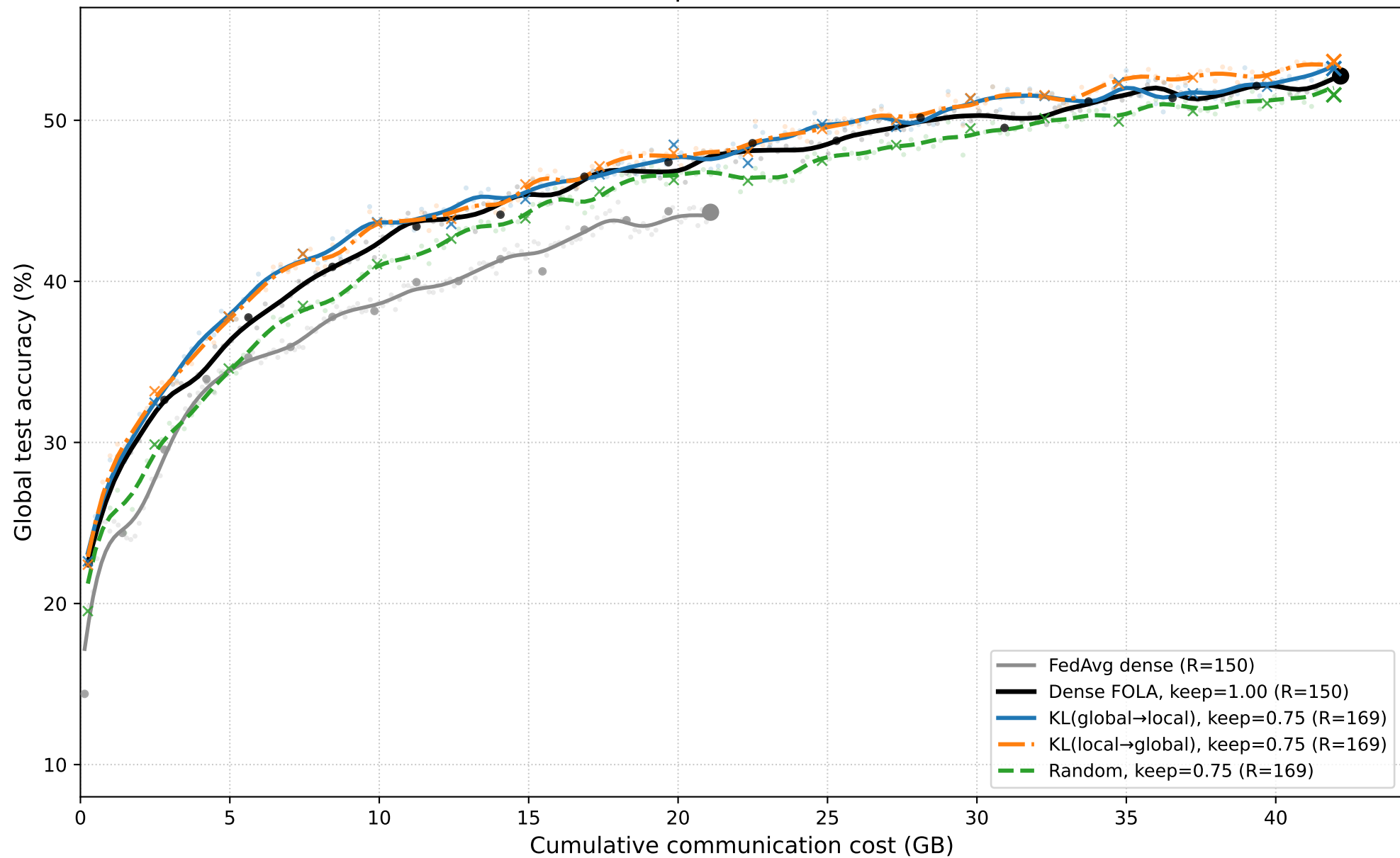
CIFAR-10 | \alpha=0.01 | local fraction=1.0 Keep ratio = 0.75
