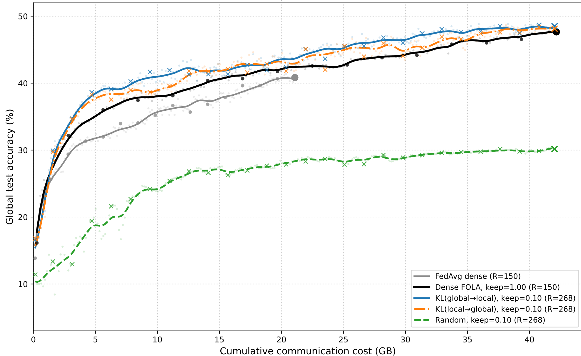
CIFAR-10 | \alpha=0.01 | local fraction=0.5 Keep ratio = 0.10
