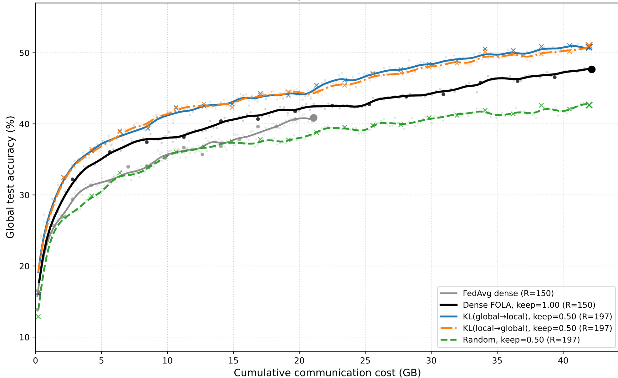
CIFAR-10 | \alpha=0.01 | local fraction=0.5 Keep ratio = 0.50
