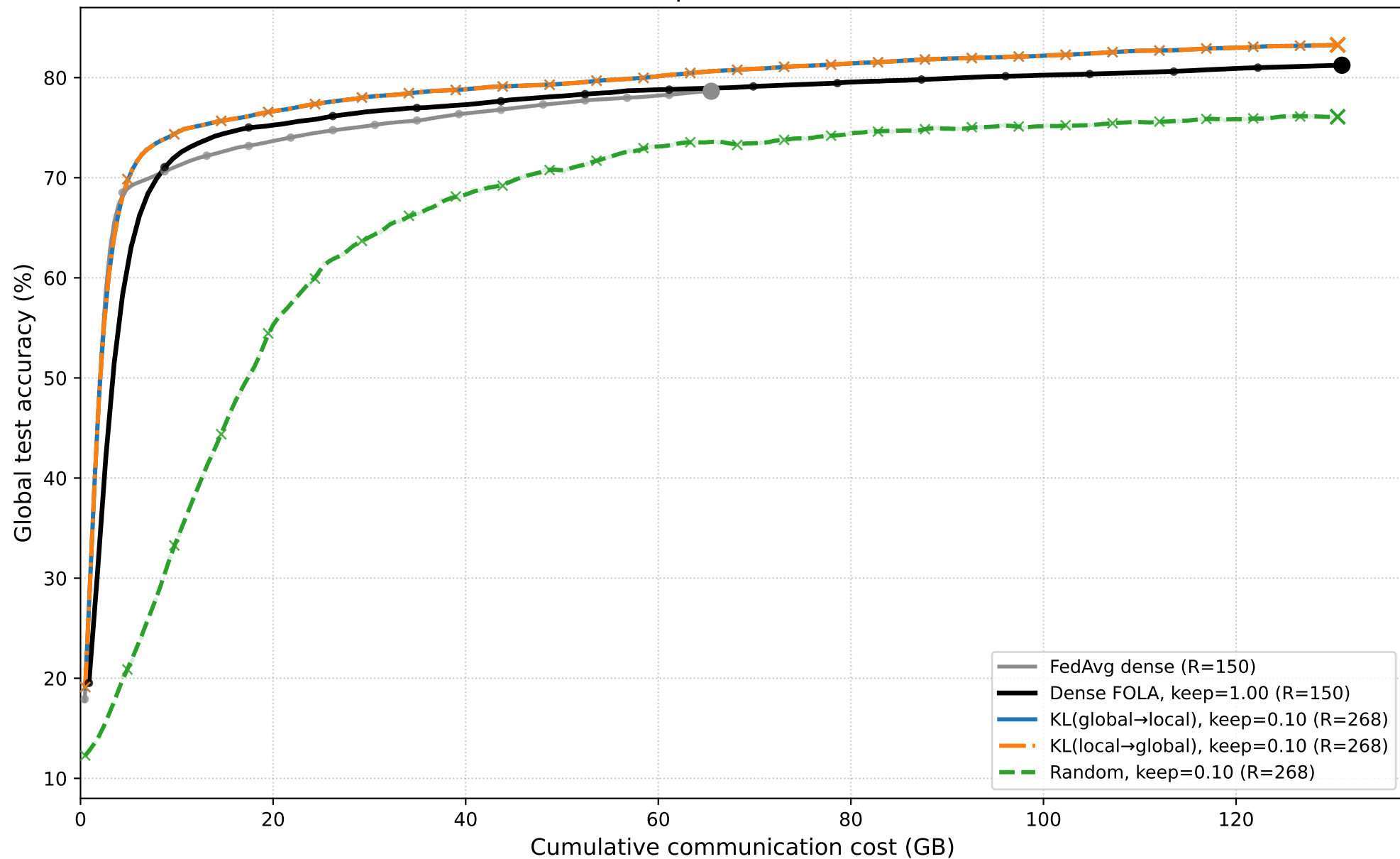
MNIST | fixed 10 samples/client | 1 class/client Keep ratio = 0.10
