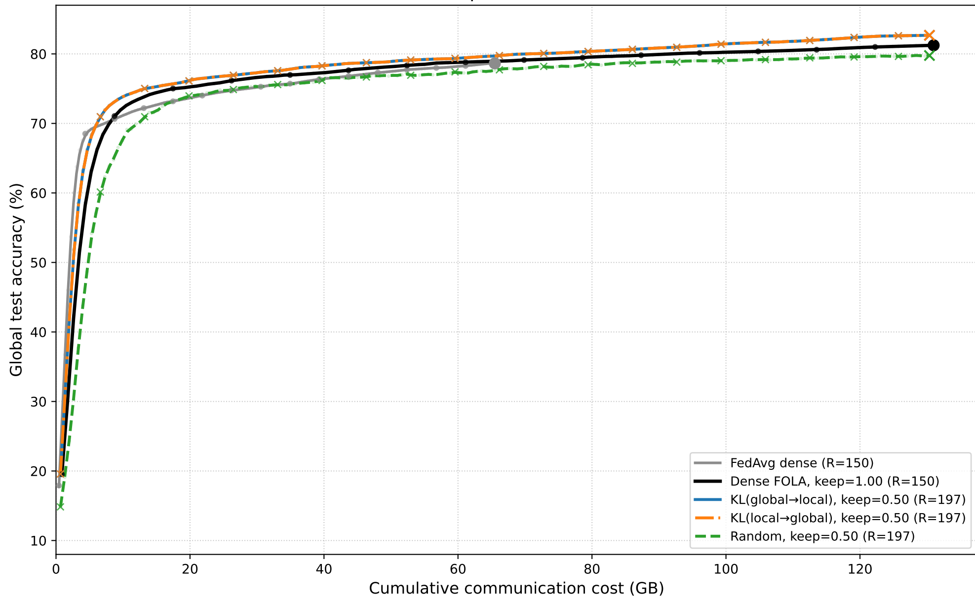
MNIST | fixed 10 samples/client | 1 class/client Keep ratio = 0.50
