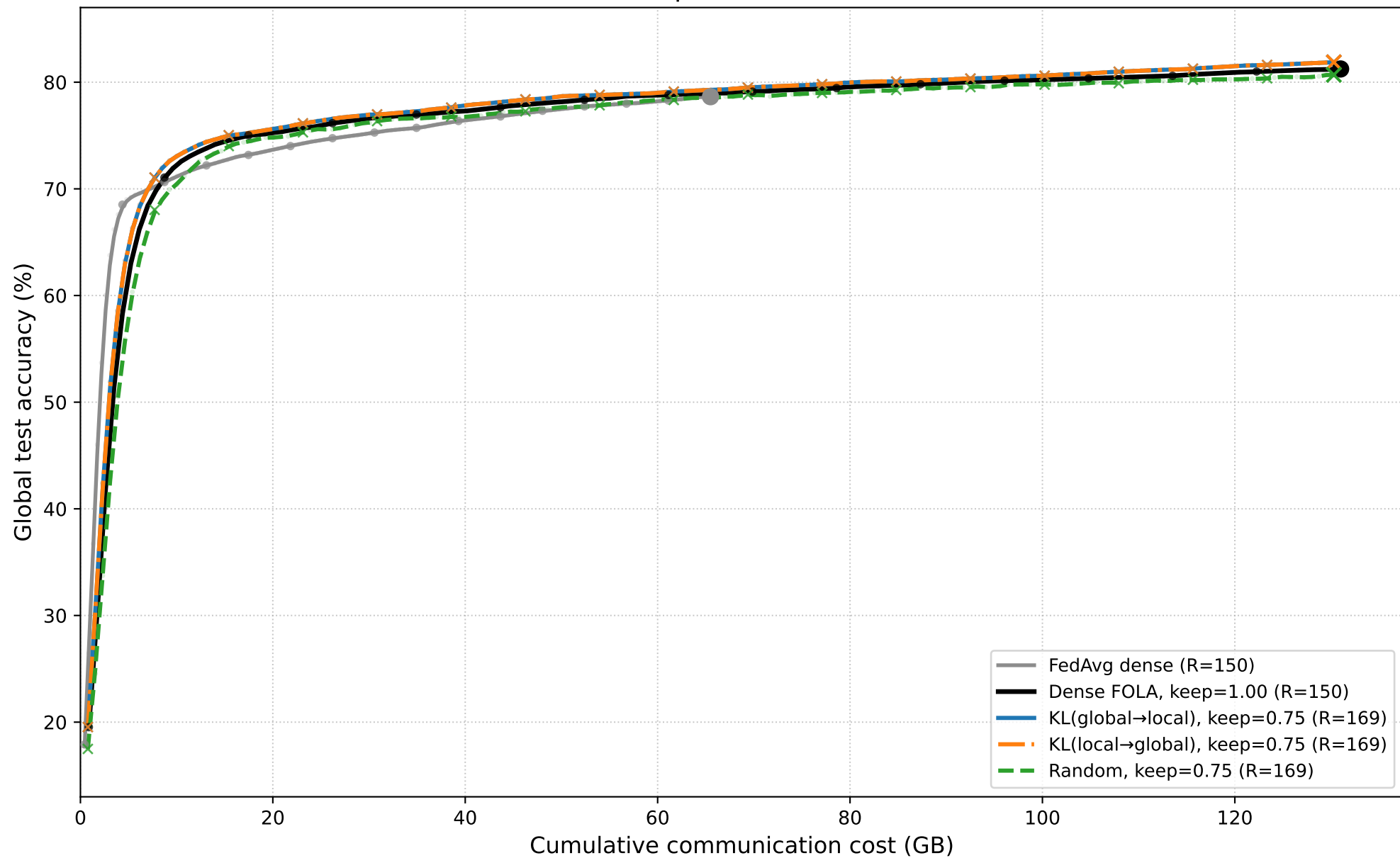
MNIST | fixed 10 samples/client | 1 class/client Keep ratio = 0.75
