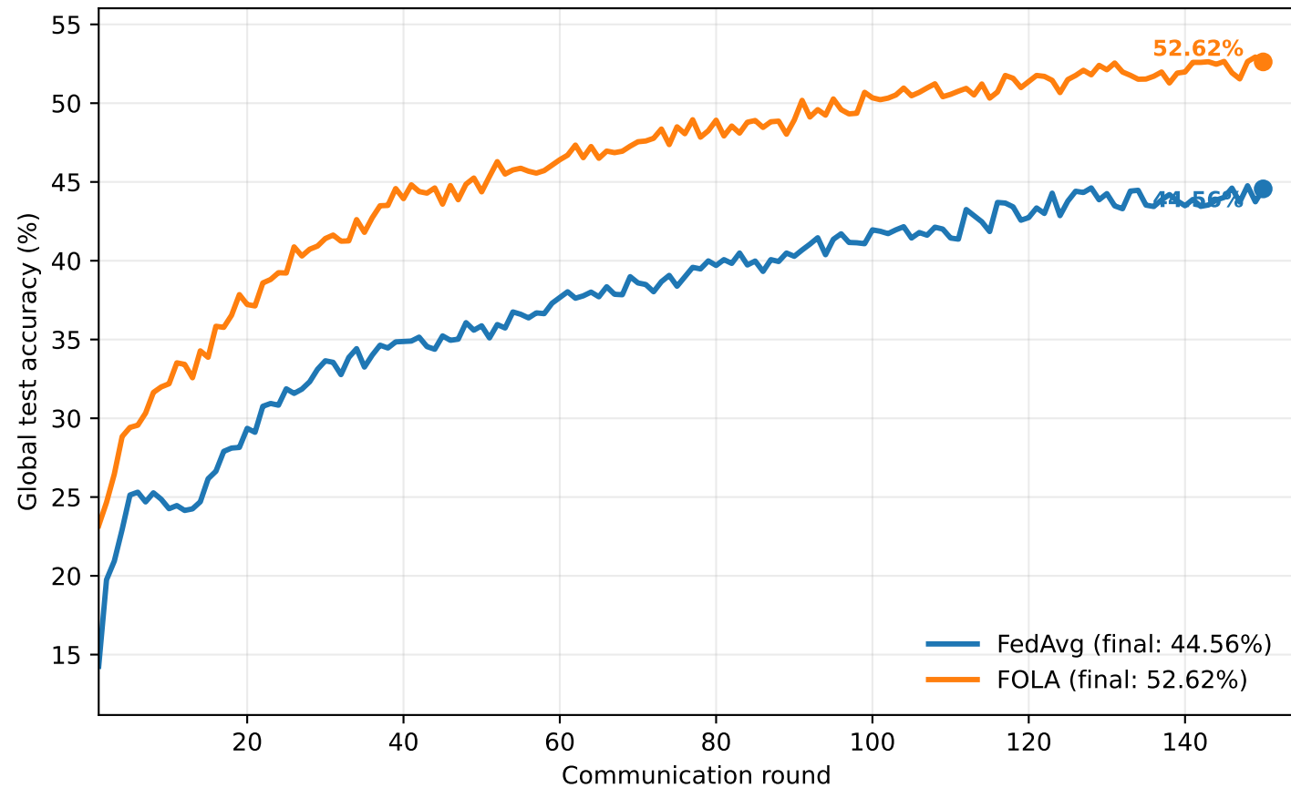
CIFAR-10 | \alpha = 0.01 ~2499 samples/client
