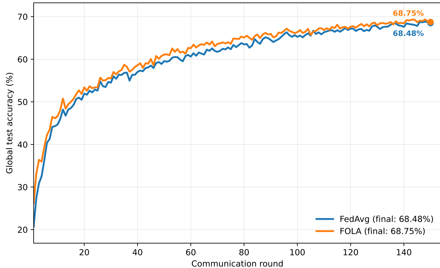
CIFAR-10 | \alpha = 0.1 ~1248 samples/client
