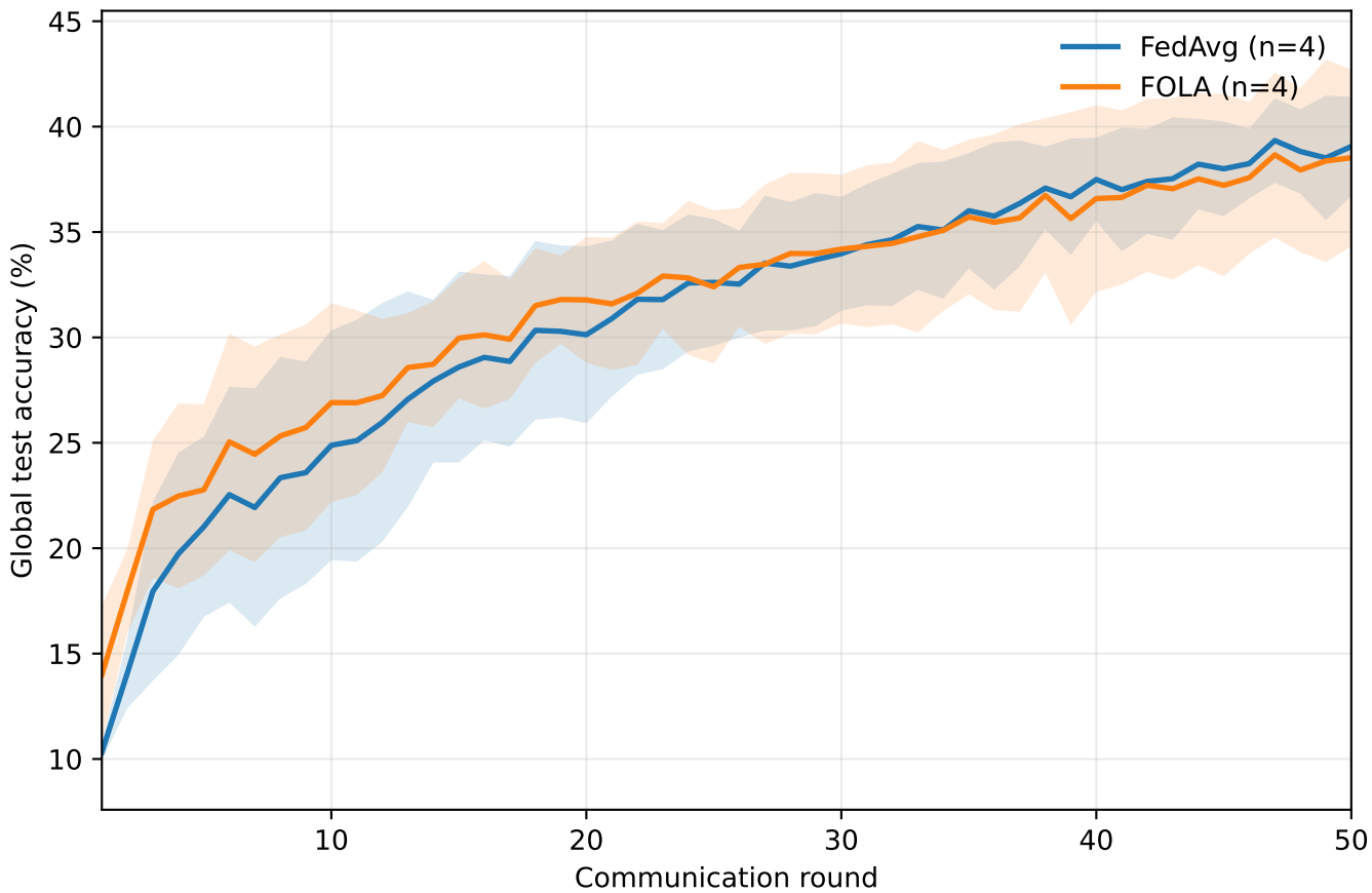
CIFAR-10 — \alpha = 0.01
