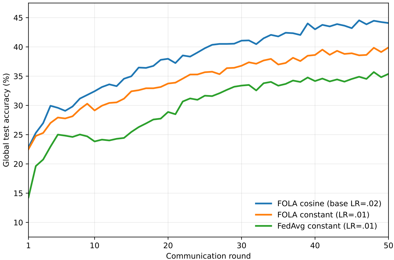
CIFAR-10 BasicCNN — \alpha = 0.01
