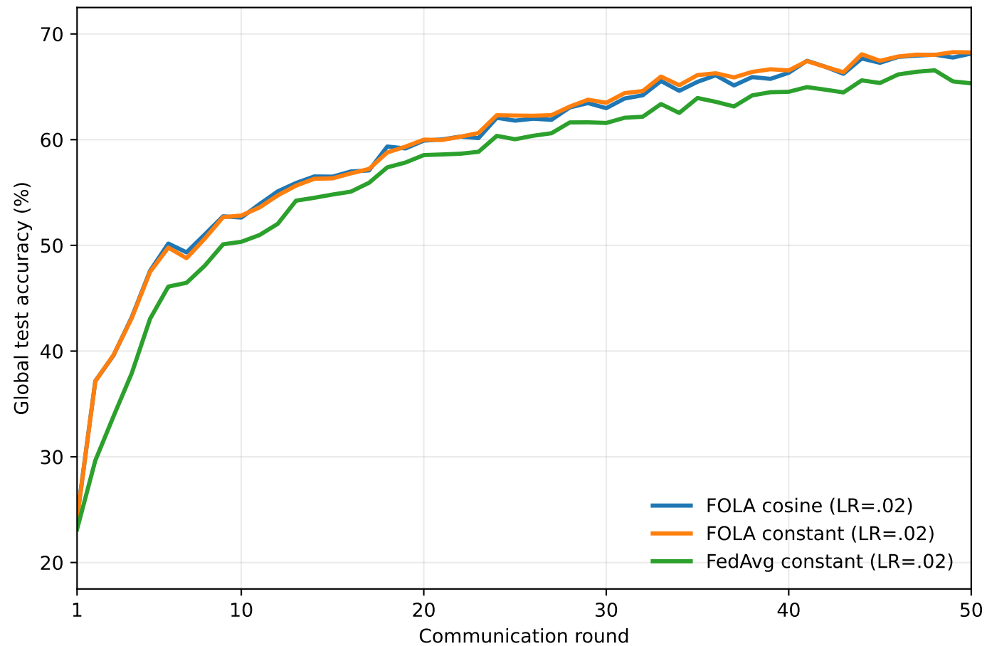
CIFAR-10 BasicCNN — \alpha = 0.1
