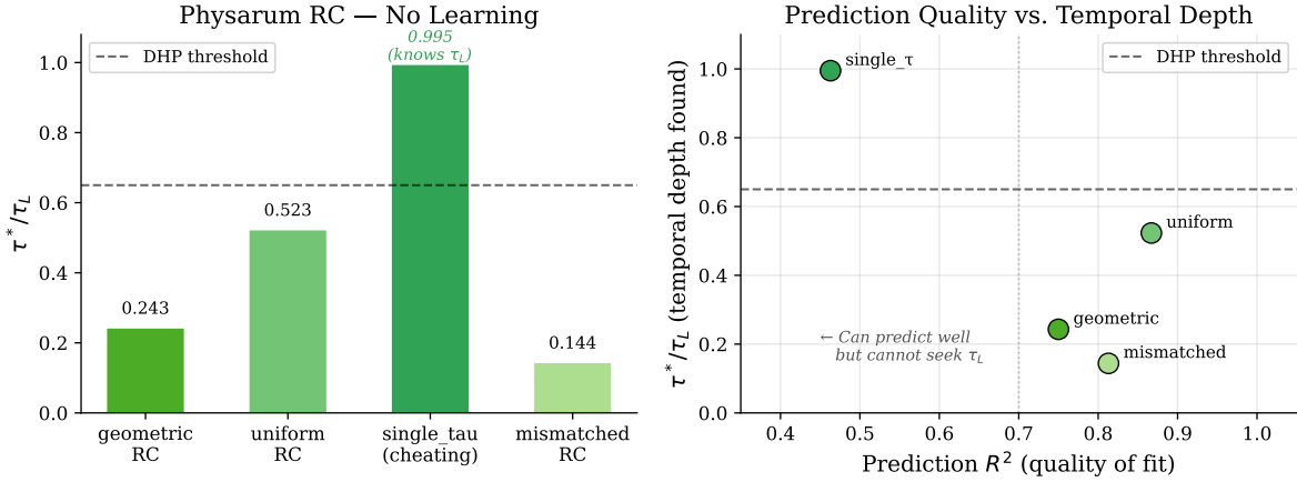
Figure 3: Physarum RC-circuit probe. Left: \tau^*/\tau_L per condition; only single_tau (oracle) clears DHP. Right: Prediction R^2 vs. temporal depth—systems can predict well ( R^2 > 0.75 ) while failing to discover \tau_L , confirming that prediction quality and temporal horizon discovery are separable.
