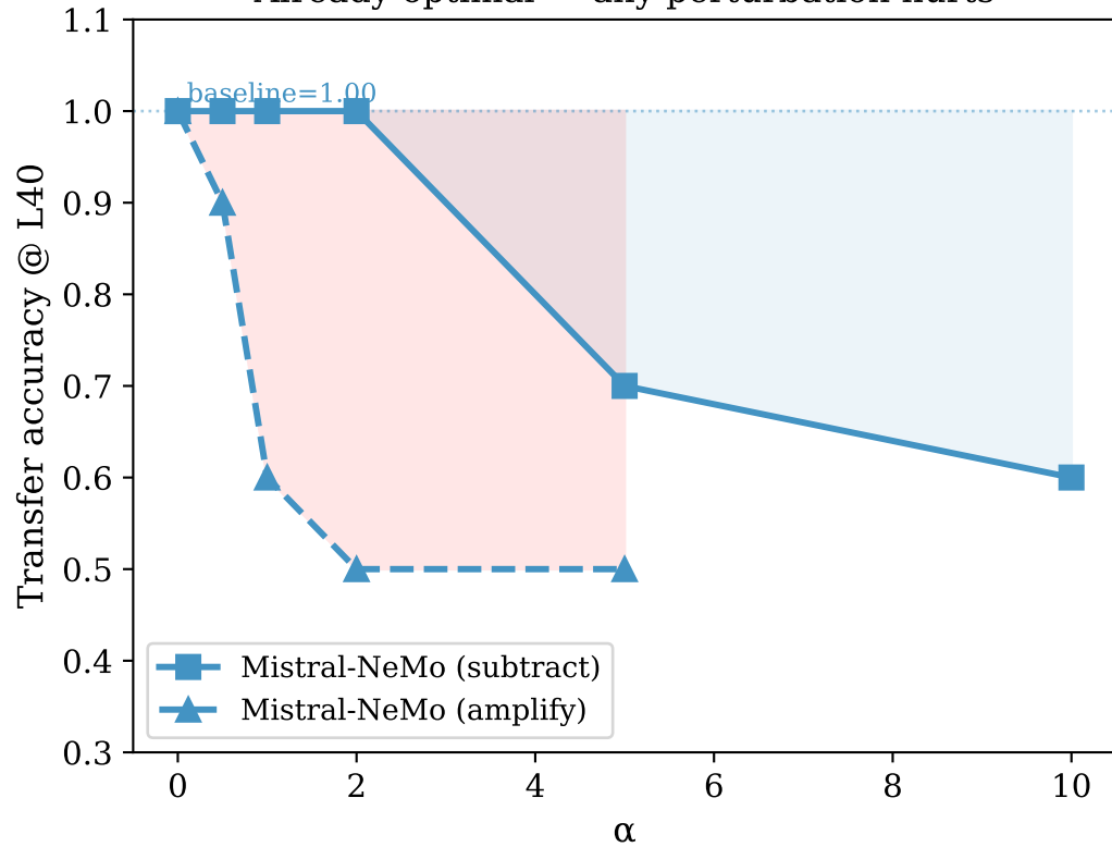
Crystallizer (Mistral-NeMo-12B) Already optimal — any perturbation hurts
