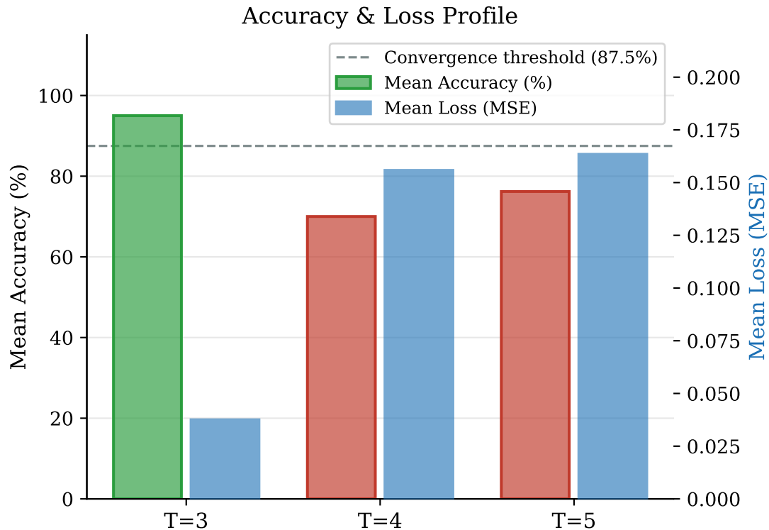
Figure 2: Archon's Discrete Trainability Cliff — 2-Qubit Q-RNN, Parity Task
