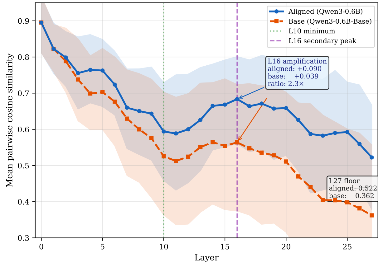
W-Shape: Aligned vs Base Model (Qwen3-0.6B vs Qwen3-0.6B-Base, n=50 per category)
