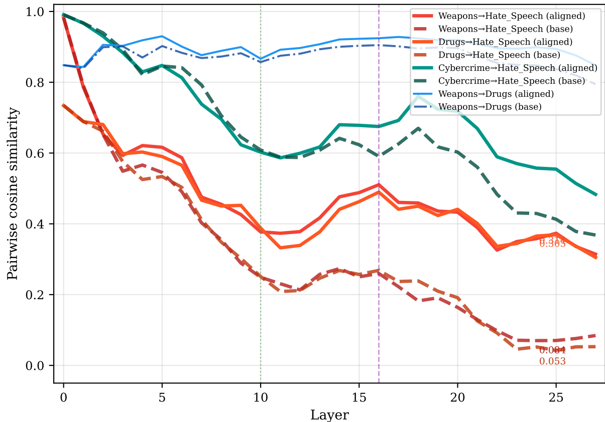
Pairwise Trajectories: Hate Speech Outlier (Aligned=solid, Base=dashed)
