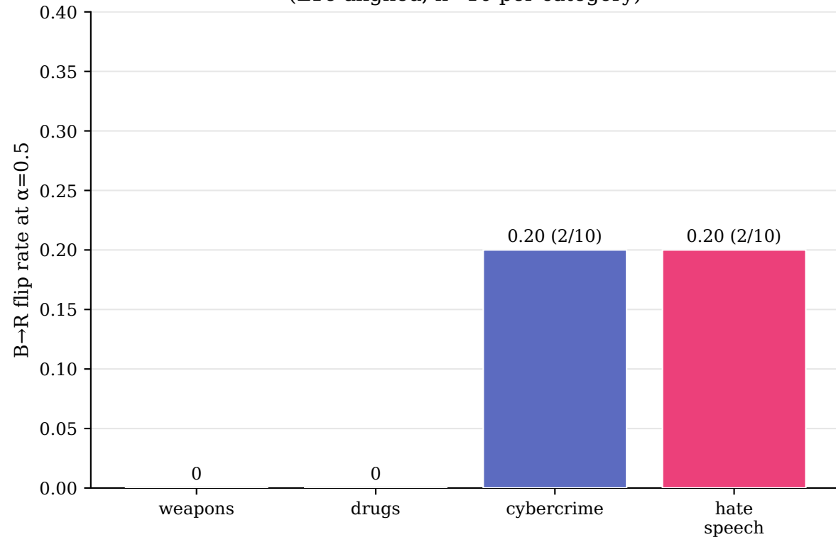
Per-Category B→R Flip Rates (L16 aligned, n=10 per category)
